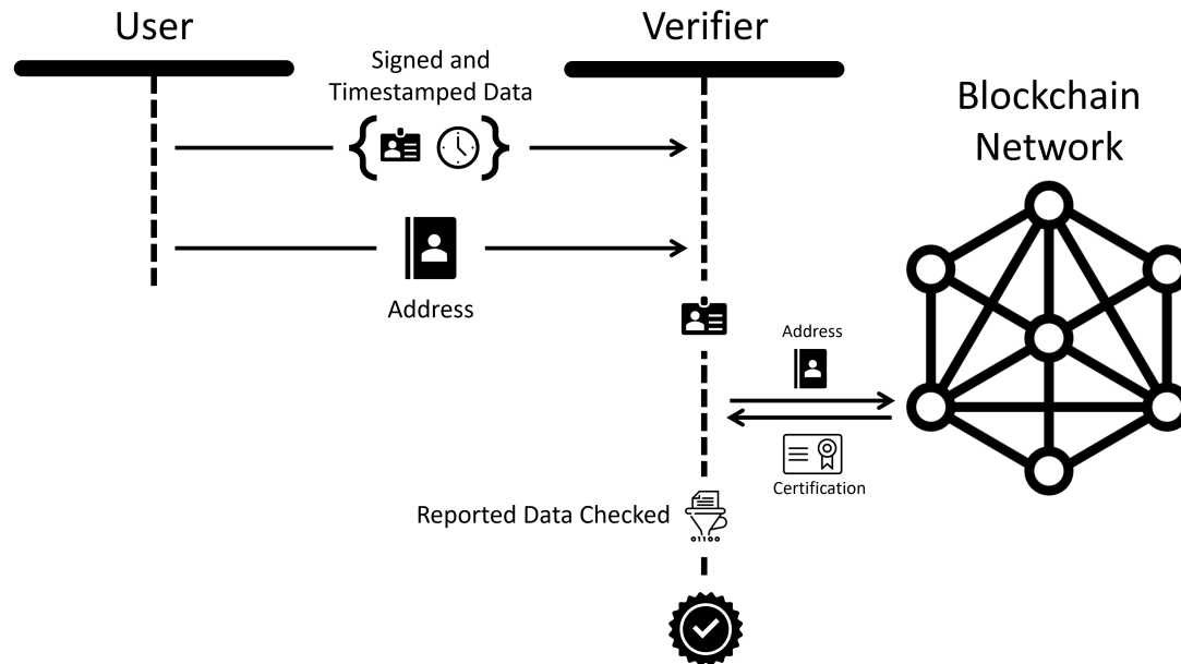
Figure 3.5: Flow chart showing how users are verified in the system.
