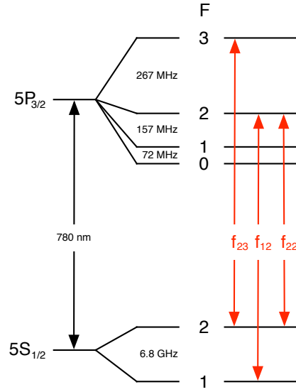
Figure 3.1: Schematic diagram of the ^{87}\text{Rb} D2 line showing the hyperfine splittings in the ground and excited states and the transitions used for laser cooling and absorption imaging. The F-number of the hyperfine levels is indicated. Transitions from the ground state hyperfine levels F to excited state hyperfine levels F' used in the experiment are labelled, specifically the principle transition f_{23} used for cooling and imaging, the repump transition f_{12} and the optical pumping transition f_{22} .
