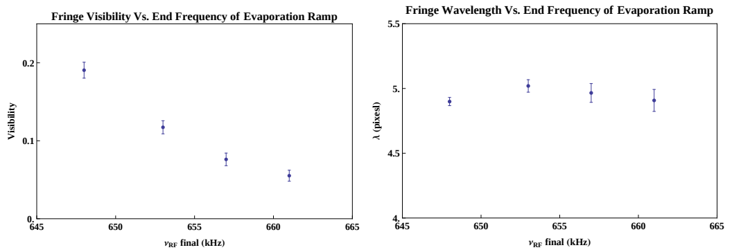
Figure 7.19: Fringe visibility and wavelength plotted against the end frequency of the evaporation ramp for the data presented in figure 7.18.
