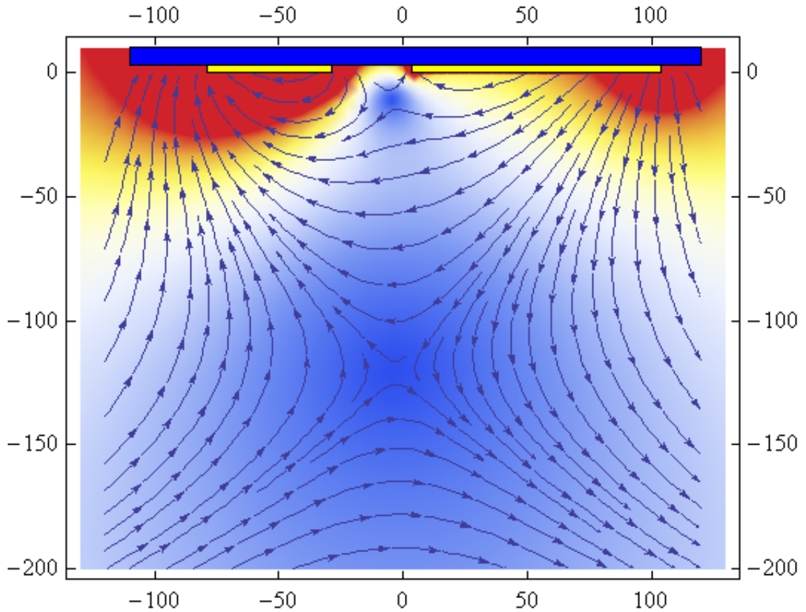
Figure 4.10: Static Trap Configuration: We use two broad wires to create the DC magnetic trap for our BEC. Wire Z3 (on the left in the figure) is 50\,\mu\text{m} wide and wire Z4 (on the right in the figure) is 100\,\mu\text{m} wide. Both wires are 3\,\mu\text{m} thick. The centre-to-centre separation of the trapping wires is 107.5\,\mu\text{m} . Note that because the trapping fields are generated by two wires, there are two local field minima. The BEC forms in the lower of the two trapping minima shown in the figure. To calculate the transverse components of our static trapping potential we use the analytical expression for the field of a wide wire given in equation (2.13). We run 1 A in each of the DC wires in series from a single current driver. In the figure the current runs into the page, and the trap is formed by adding a bias field along the x -axis of 27.5 G. The trap forms 132\,\mu\text{m} below the surface of the chip. The finite thickness of the trapping wires makes no significant contribution to the trapping potential. The quadrupole field around the trap minimum is slightly rotated because of the asymmetry between the two trapping wires.
